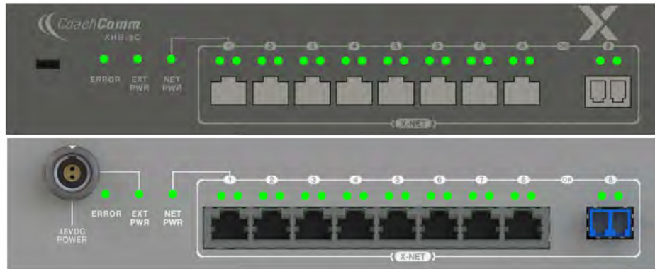
Figure 154: X-System Hub Front and Rear View
