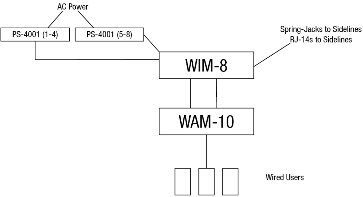
Figure 7: Wired Press Box Unit Block Diagram
