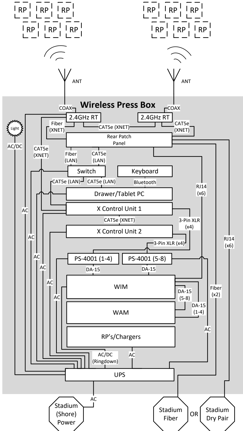
Figure 128: Wireless Press Box Unit (WPB1) Block Diagram
