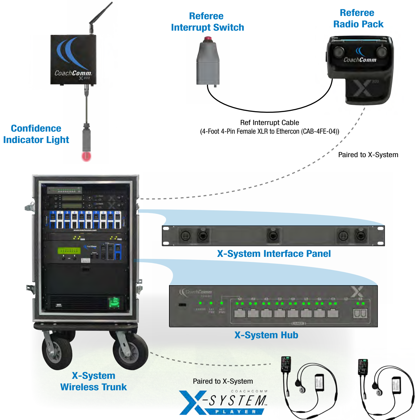
Figure 137: CoachComm X-System Player Block Diagram (Single Wirelless Referee Interrupt Configuration)
