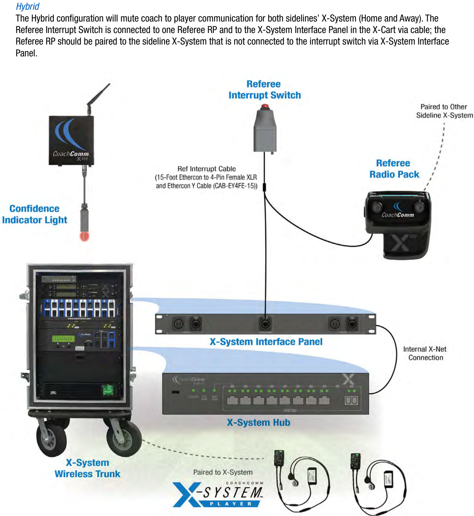
Figure 153: X-System Player Block Diagram (Hybrid Referee Interrupt Configuration)
