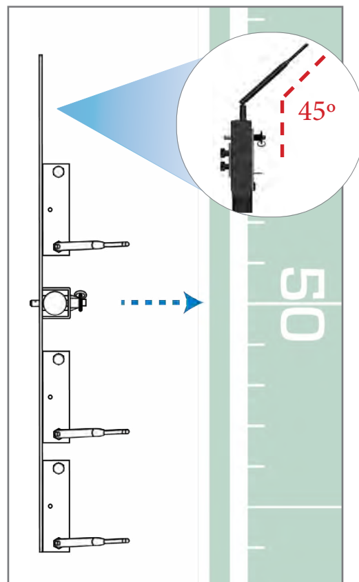
Figure 111: Top View of RT Bracket and Antenna Direction
