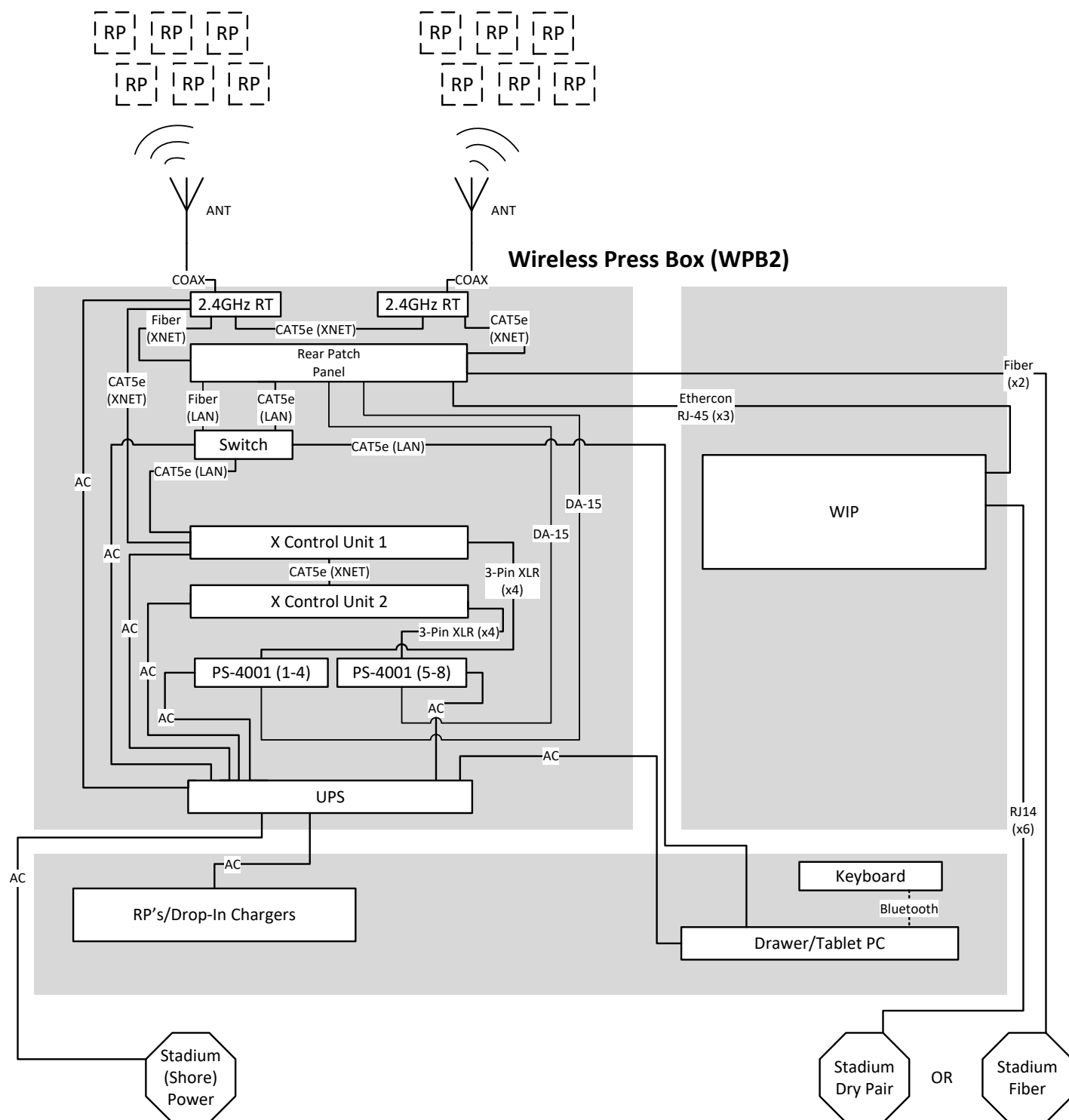
Figure 132: Wireless Press Box Unit (WPB2) Block Diagram
