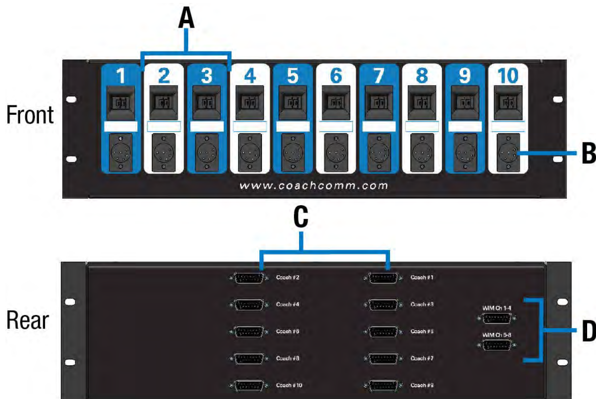
Figure 28: WAM 10 Overview
