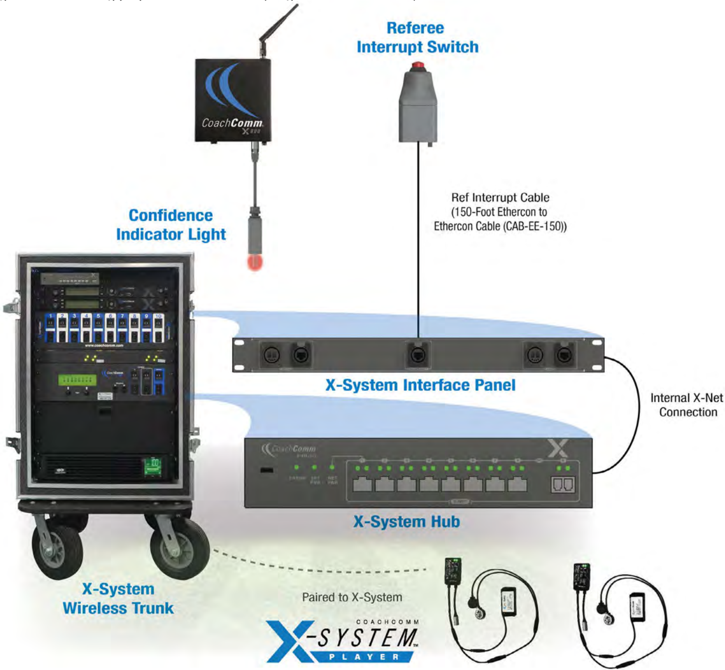
Figure 151: X-System Player Block Diagram (Wired Referee Interrupt Configuration)
