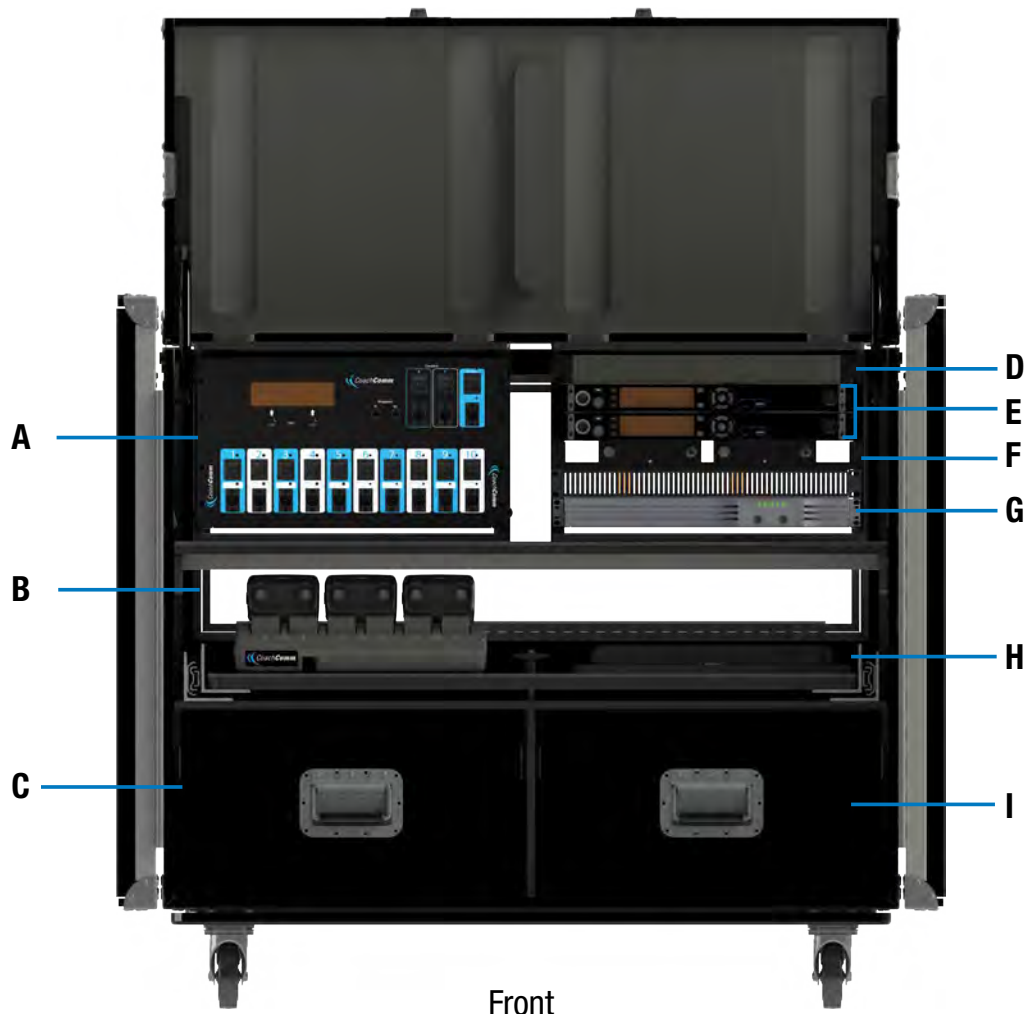
Figure 133: Wireless Press Box Unit (WPB2) Front View
