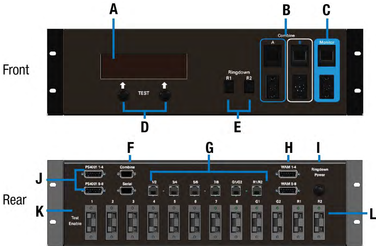
Figure 23: WIM 8 Overview
