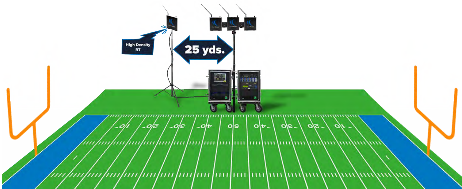
Figure 156: High Density Mode Radio Transceiver Deployment
