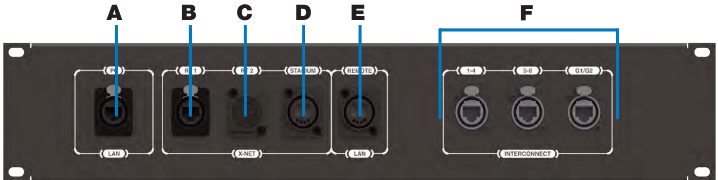
Figure 135: Wireless Press Box (WPB2) Rear Patch Panel
