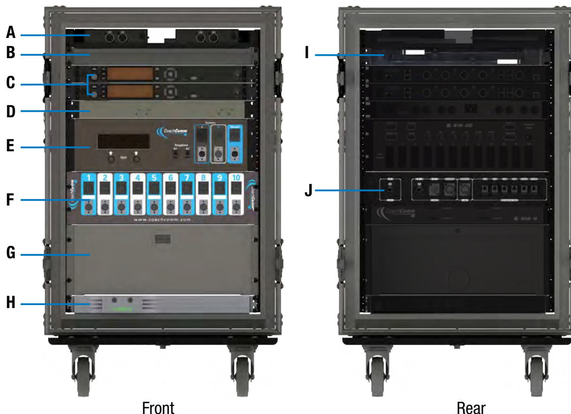
Figure 129: Wireless Press Box Unit (WPB1) Overview
