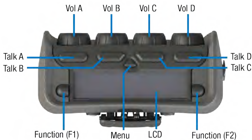
Figure 38: XRP-44
