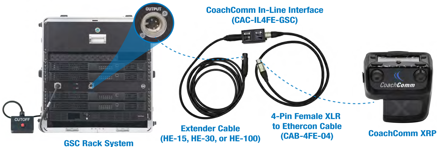
Figure 170: CoachComm to GSC Connection Diagram
