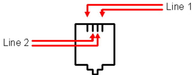
Figure 139: RJ-14 Wiring
