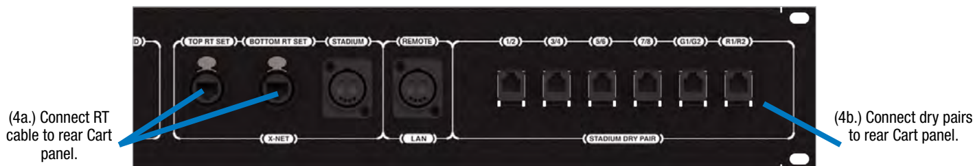
Figure 14: Patch Panel RT Cable and Dry Pair Ports
