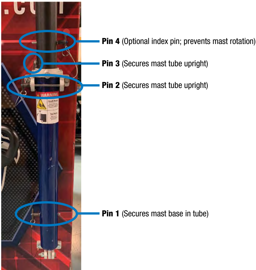
Figure 122: RT Mast Pin Locations
