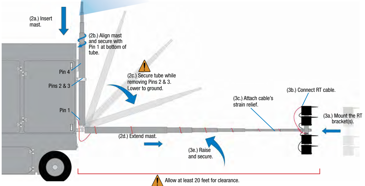
Figure 13: Sideline Cart RT Mast Setup
