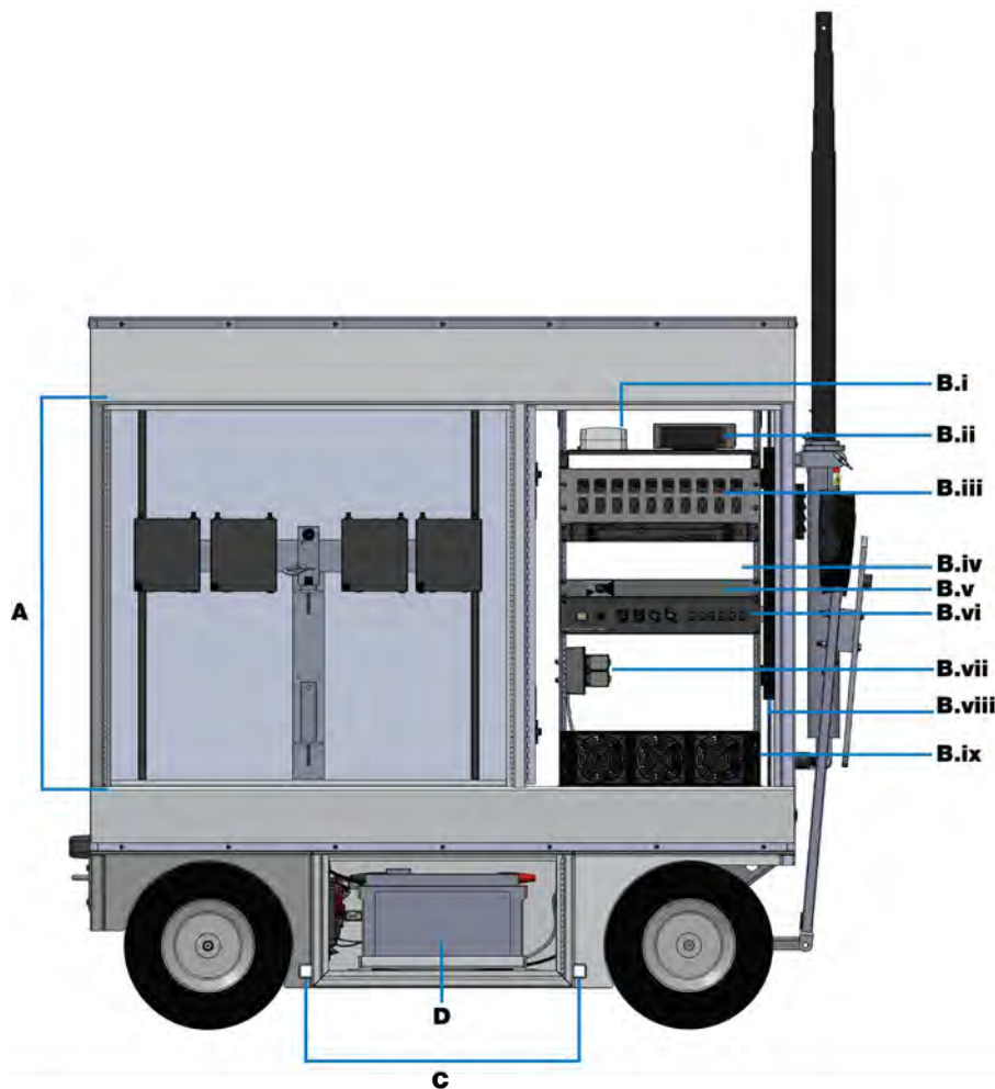
Figure 19: Sideline Cart Front View
