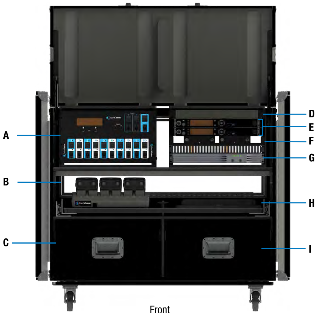
Figure 146: Wireless Press Box Unit (WPB2) Front View
