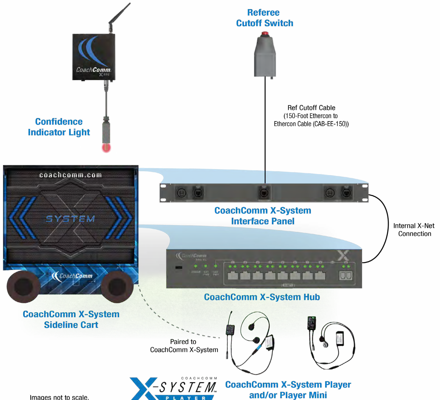
Figure 167: CoachComm X-System Player Block Diagram (Wired Referee Cutoff Configuration)
