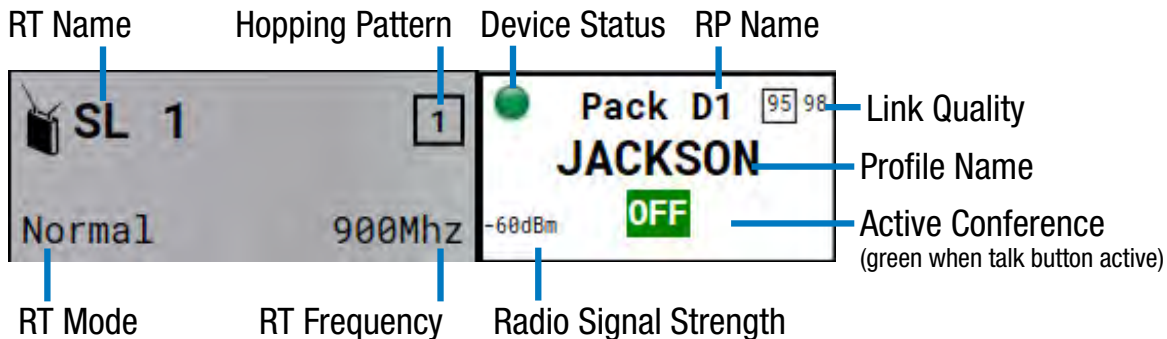
Figure 83: Radio Transceiver View Detail
