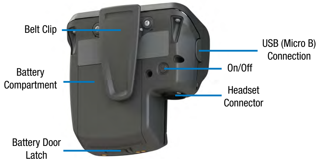
Figure 51: Radio Pack Rear View
