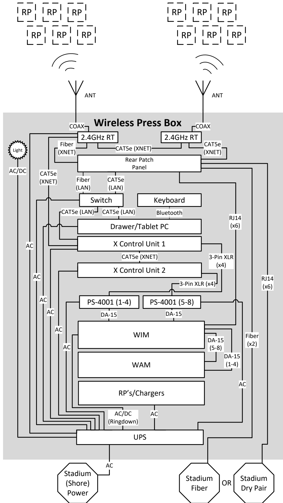
Figure 141: Wireless Press Box Unit (WPB1) Block Diagram
