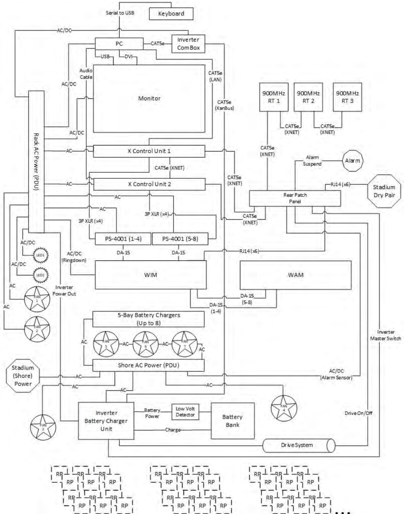
Figure 10: Sideline Cart Block Diagram (with Hub & Interface Panel)
