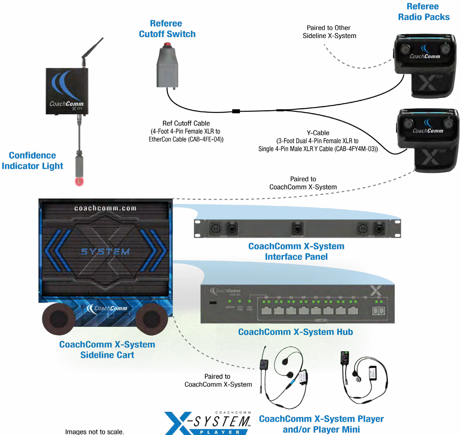
Figure 168: CoachComm X-System Player Block Diagram (Dual Wireless Referee Cutoff Configuration)
