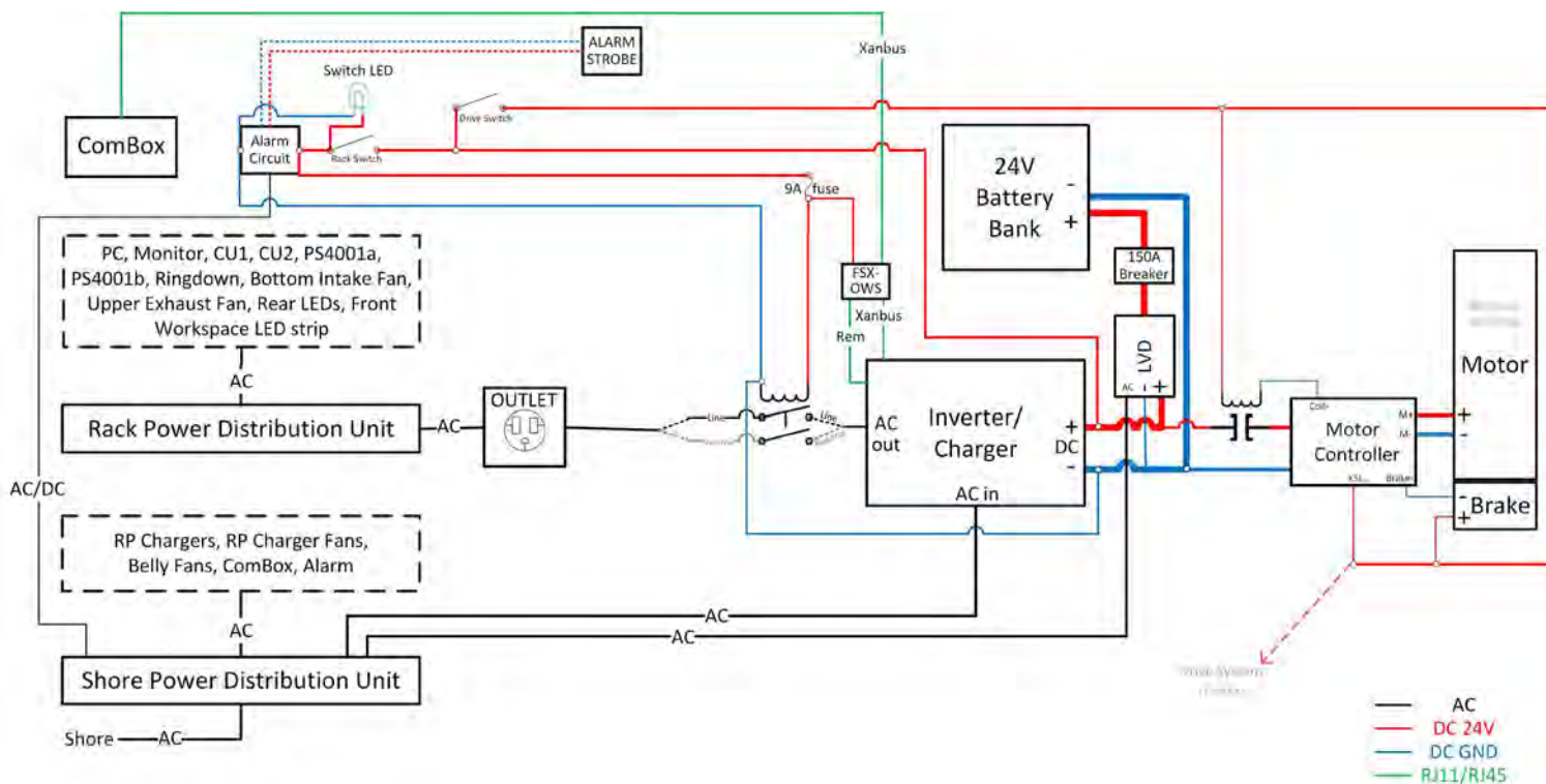
Figure 37: Sideline Cart Power Management Block Diagram
