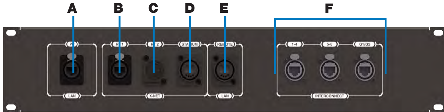
Figure 148: Wireless Press Box (WPB2) Rear Patch Panel
