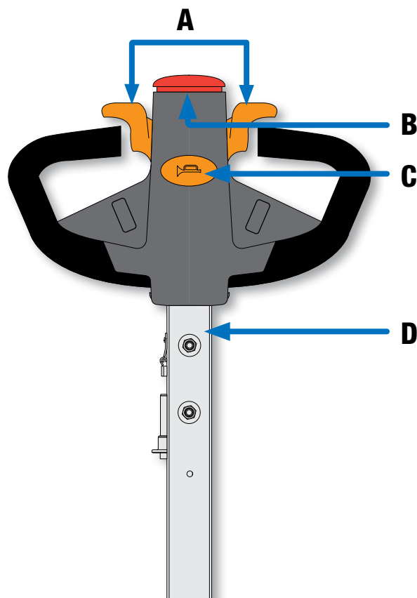
Figure 28: Drive Handle Controls
