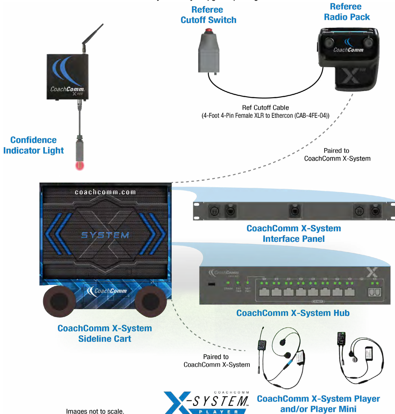
Figure 150: CoachComm X-System Player Block Diagram (Single Wireless Referee Cutoff Configuration)
