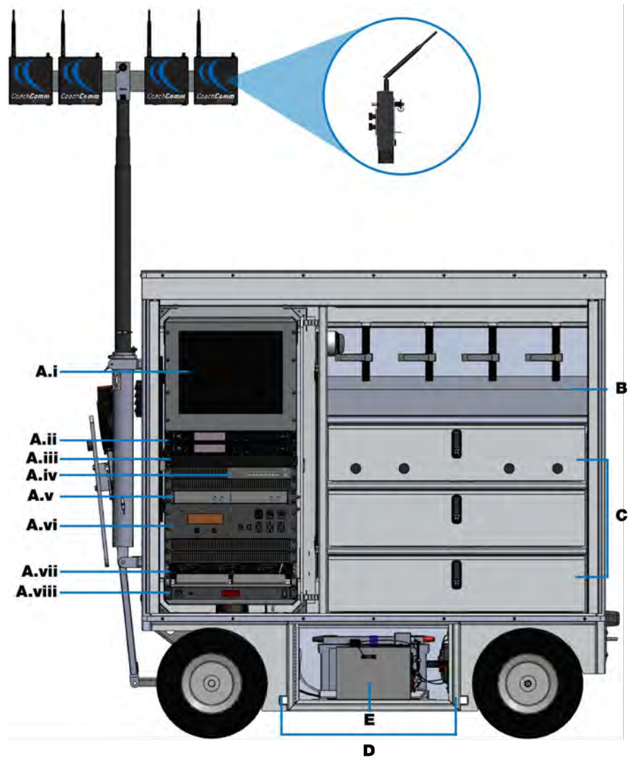
Figure 18: Sideline Cart Front View
