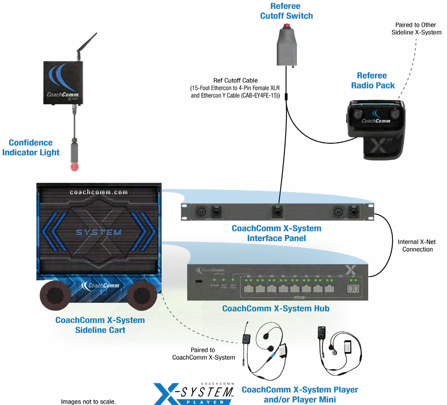
Figure 169: CoachComm X-System Player Block Diagram (Hybrid Referee Cutoff Configuration)
