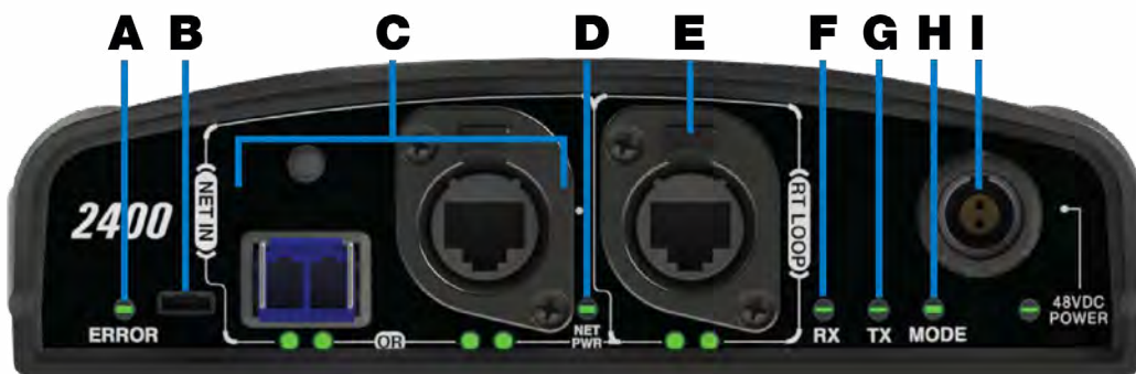
Figure 47: IP-Rated Radio Transceiver Bottom View
