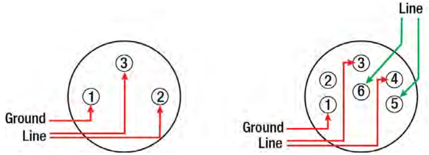
Figure 138: XLR Terminations
