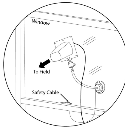
Window Mount
