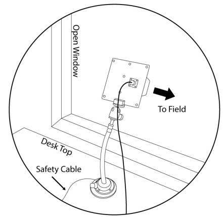
Desk Mount
