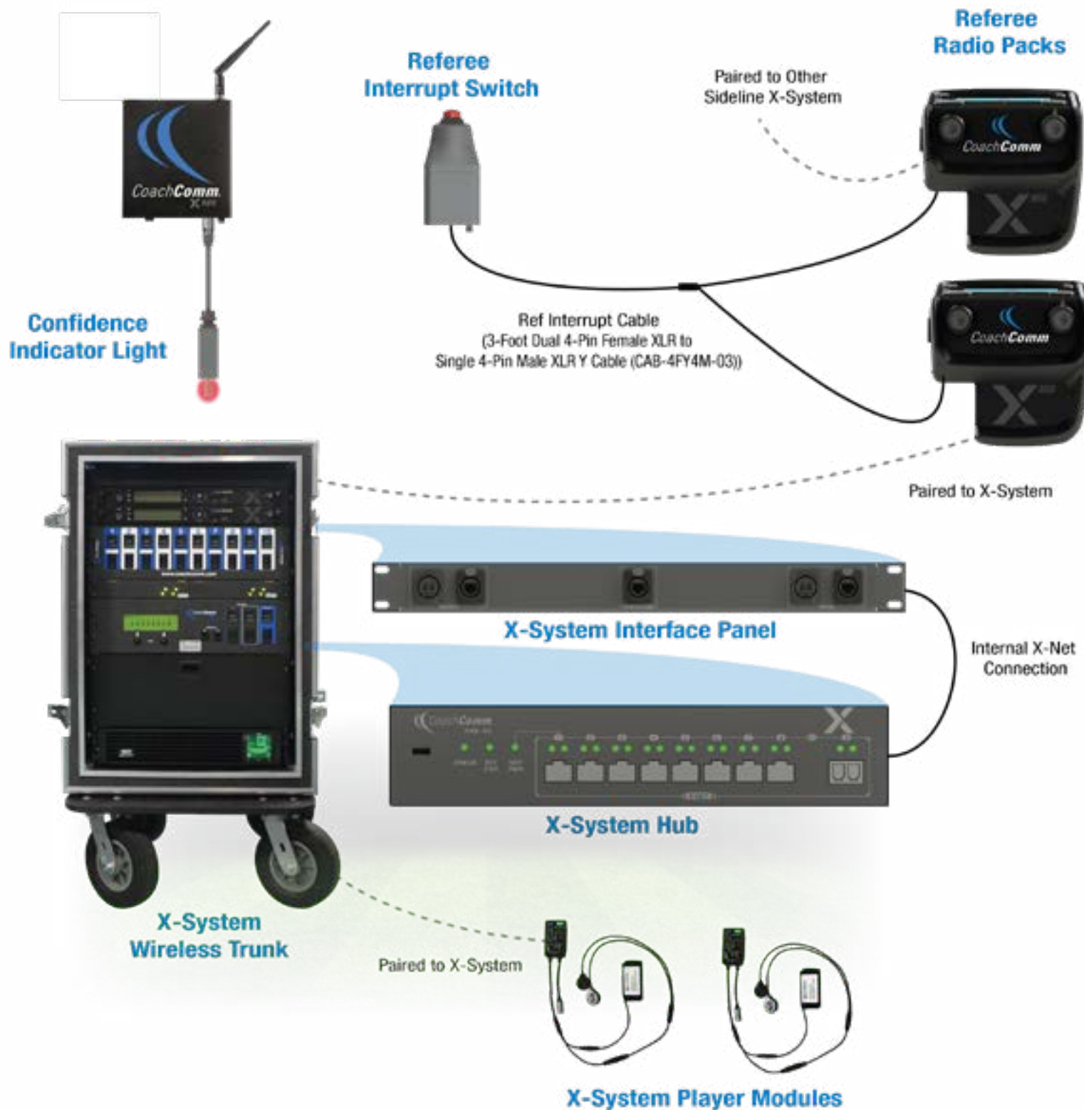
Figure 143: X-System Player Block Diagram (Dual Wireless Referee Interrupt Configuration)
