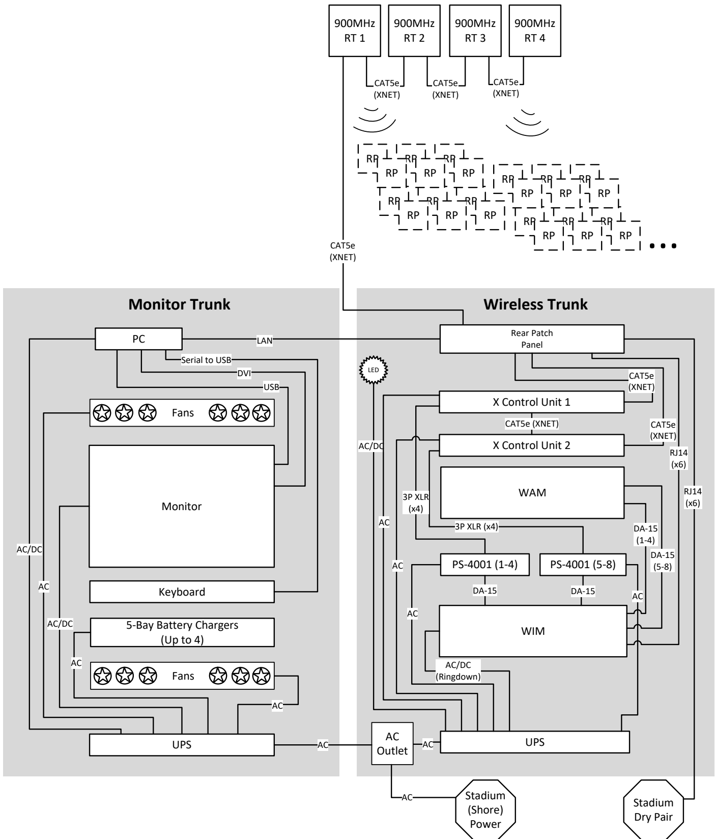
Figure 8: Sideline Trunks Block Diagram
