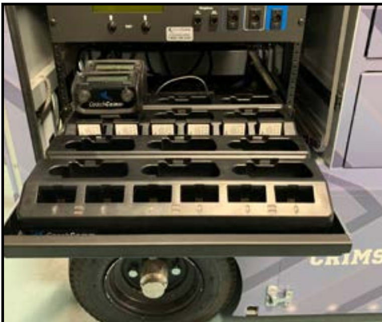
Figure 43: 6+6 Drop-In RP and Battery Chargers (shown in X-Cart)
