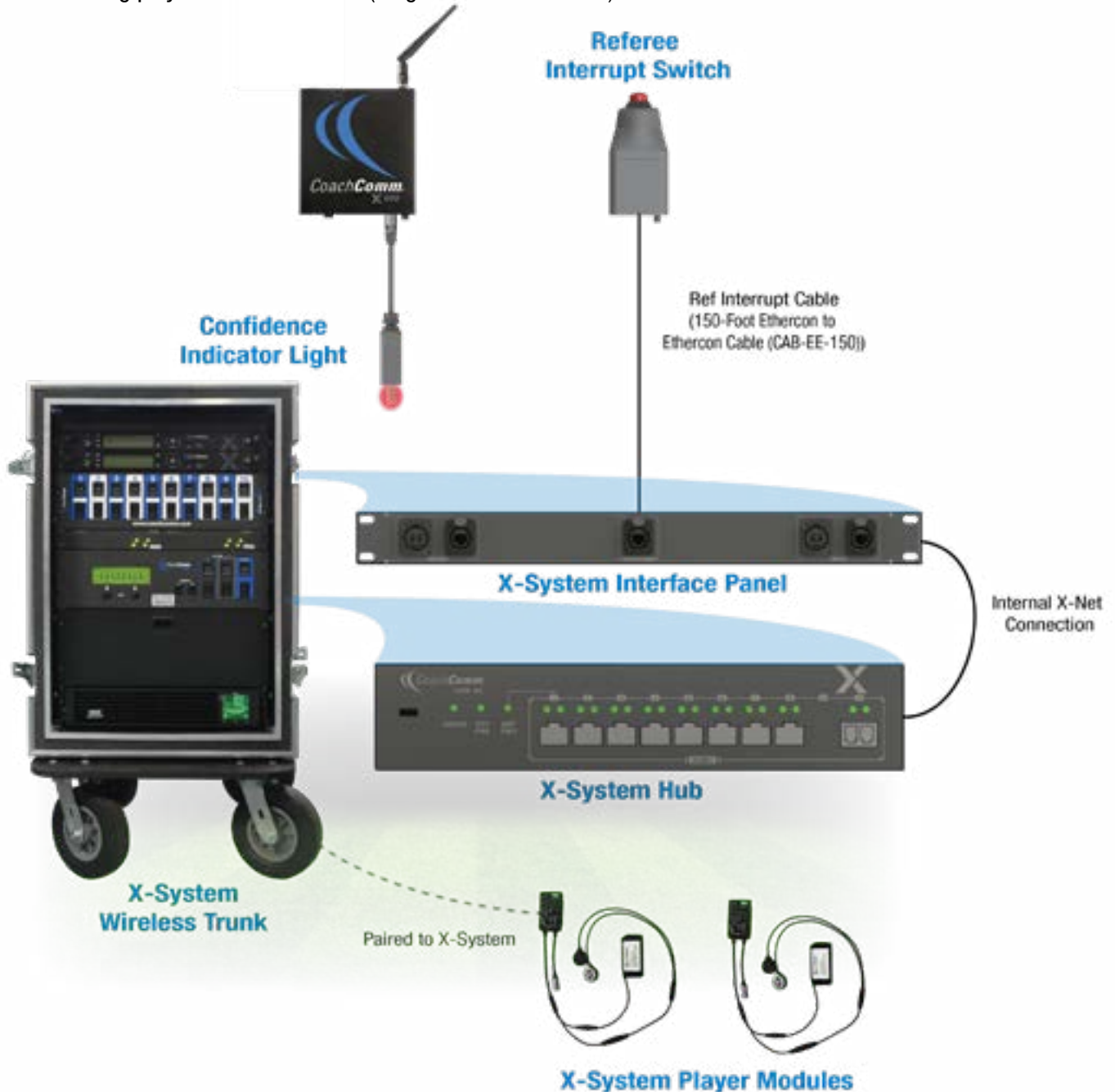
Figure 142: X-System Player Block Diagram (Wired Referee Interrupt Configuration)
