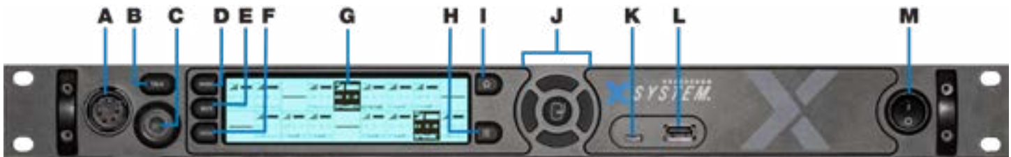
Figure 29: Control Unit Front View
