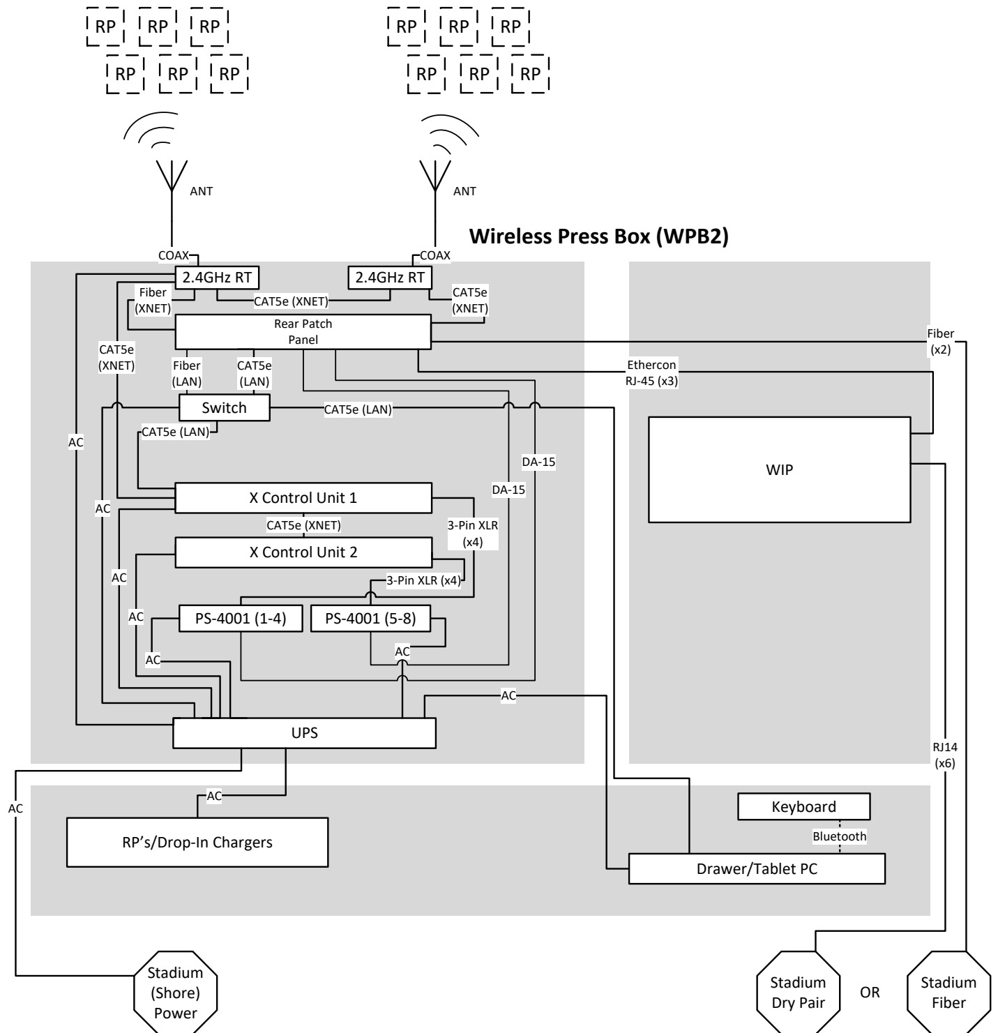
Figure 129: Wireless Press Box Unit (WPB2) Block Diagram
