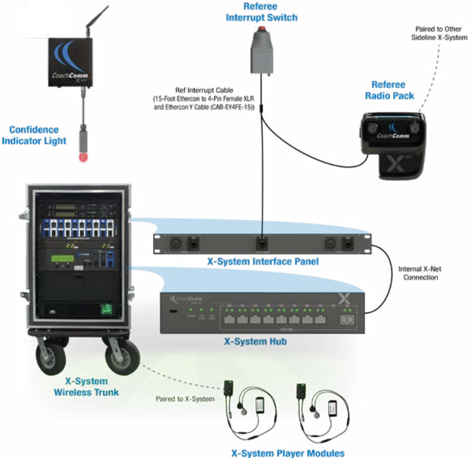
Figure 144: X-System Player Block Diagram (Hybrid Referee Interrupt Configuration)
