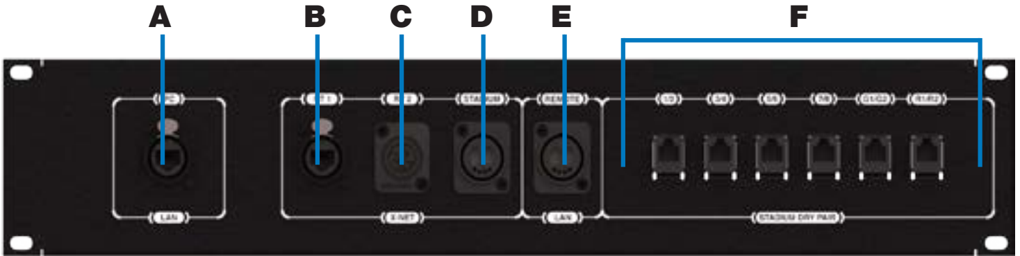
Figure 127: Wireless Press Box (WPB1) Rear Patch Panel
