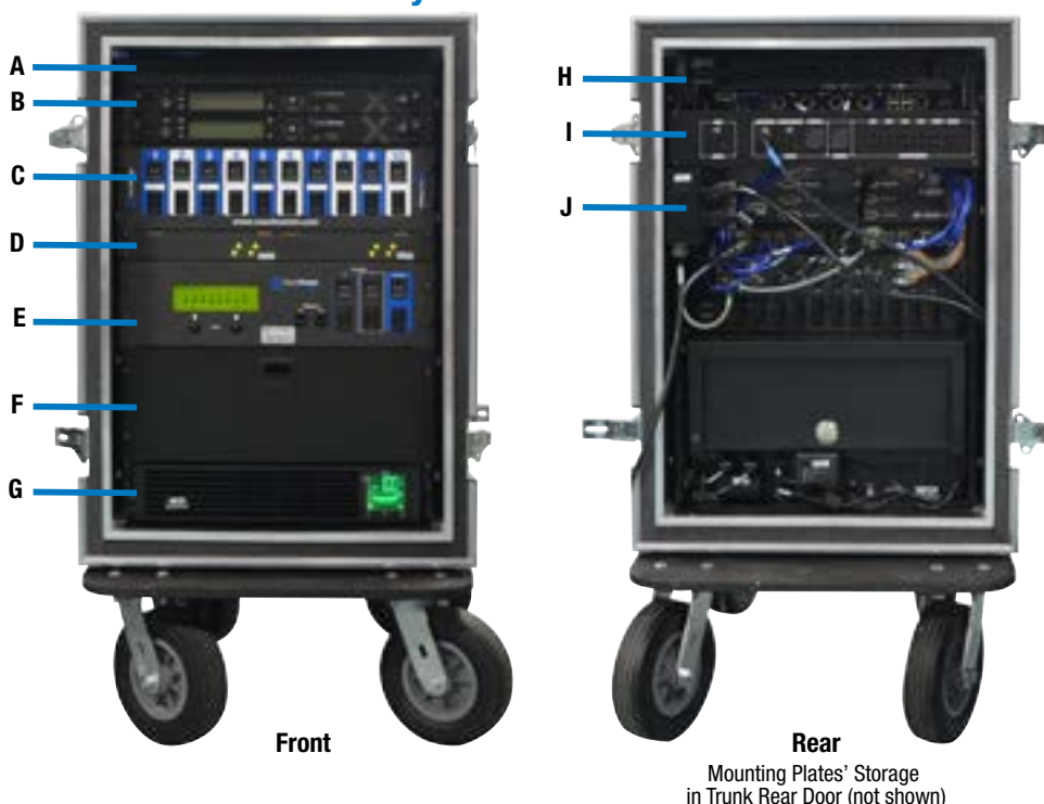
Figure 16: X-System Wireless Trunk
