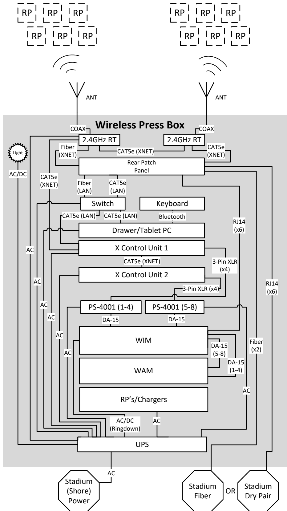
Figure 125: Wireless Press Box Unit (WPB1) Block Diagram
