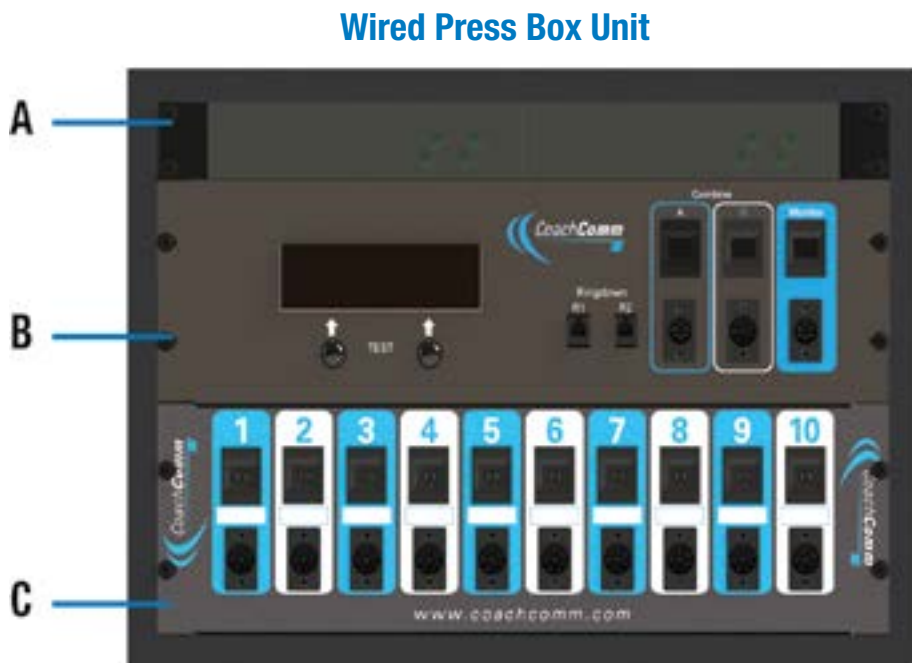
Figure 20: Wired Press Box Unit Front View
