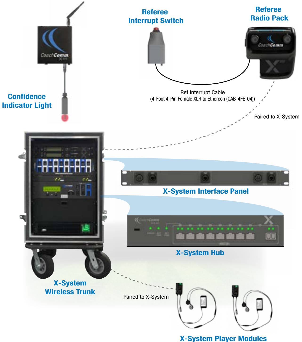
Figure 134: X-System Player Block Diagram (Single Wirelsss Referee Interrupt Configuration)
