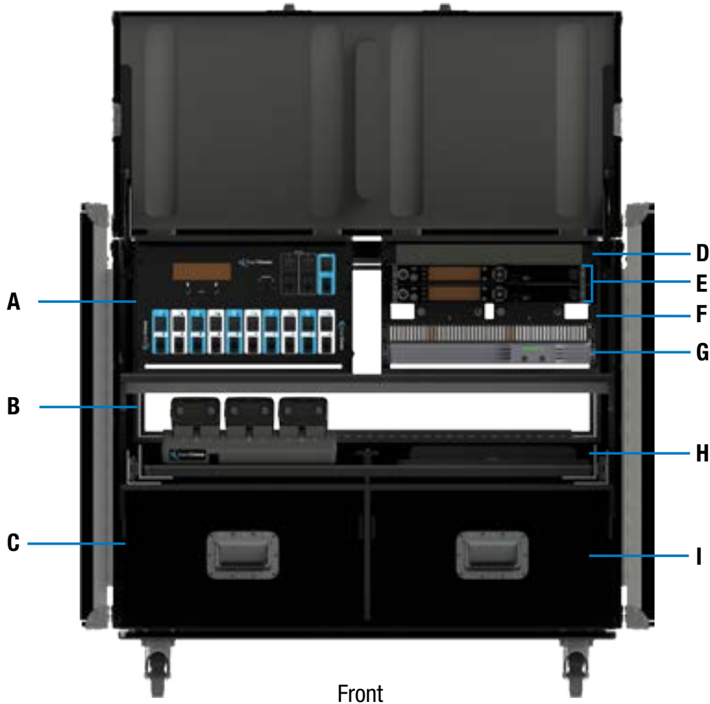
Figure 130: Wireless Press Box Unit (WPB2) Front View
