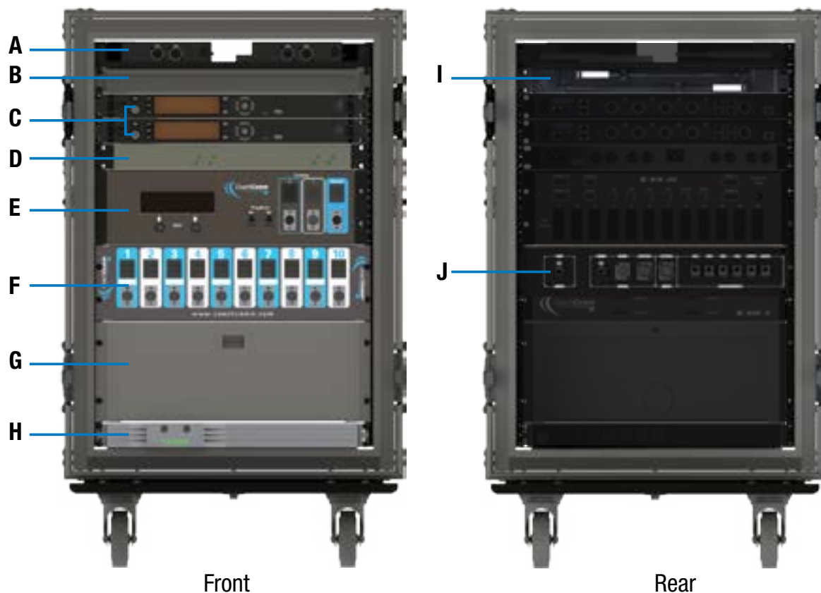
Figure 126: Wireless Press Box Unit (WPB1) Overview
